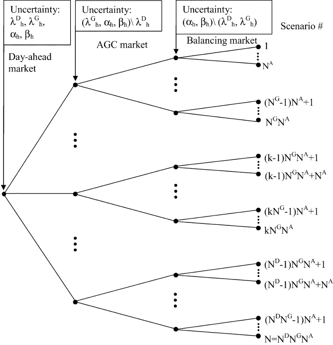
Fig. 2. Scenario tree.
